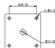
Head panel installation size
